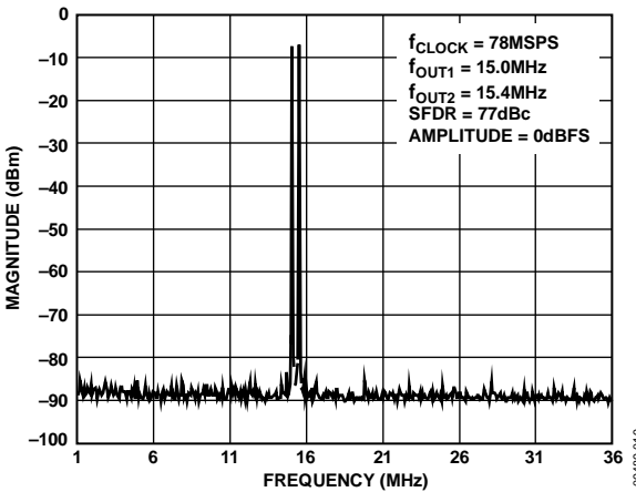
Figure 19. Dual-Tone SFDR
