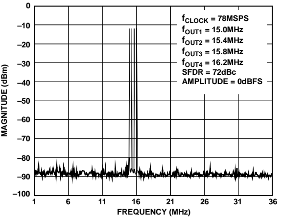
Figure 20. Four-Tone SFDR
