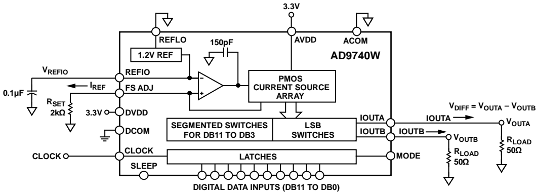
Figure 21. Simplified Block Diagram
