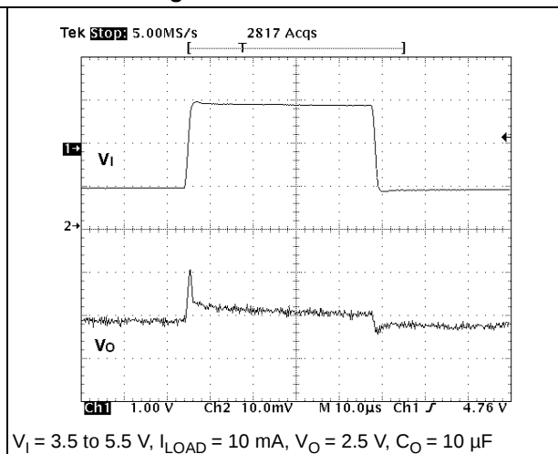
Figure 16. Line transient
