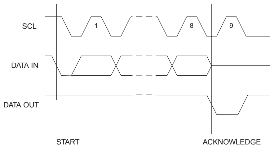
Figure 11-5. Output Acknowledge
