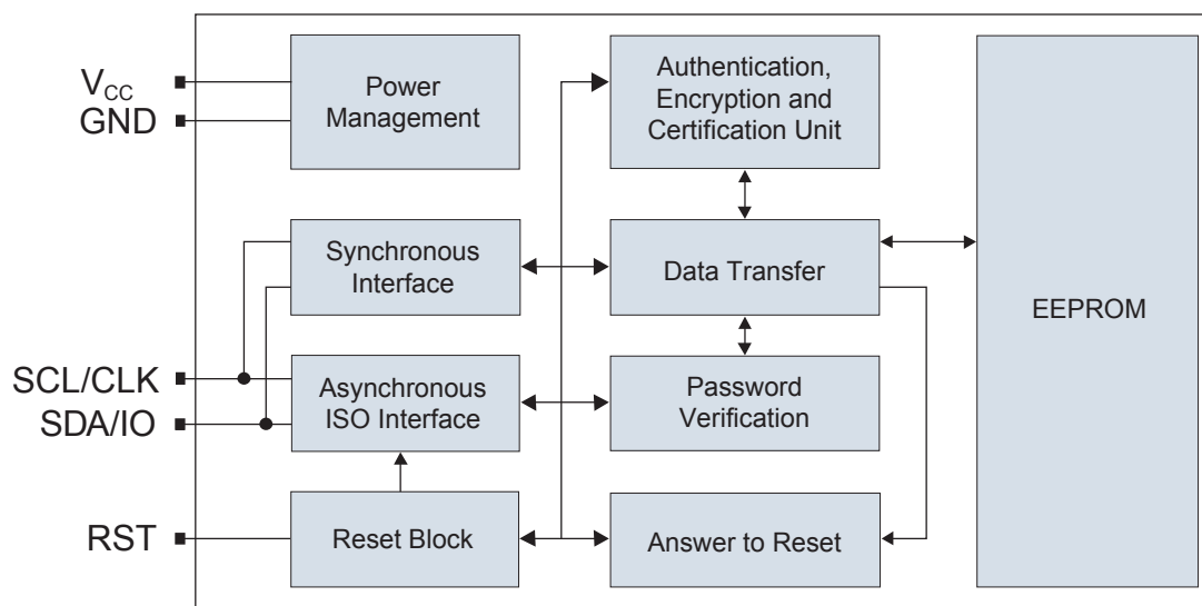
Figure 2-1. Block Diagram
