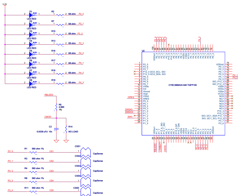
Figure 4-16. PCB Schematic for CapSense Slider Project
