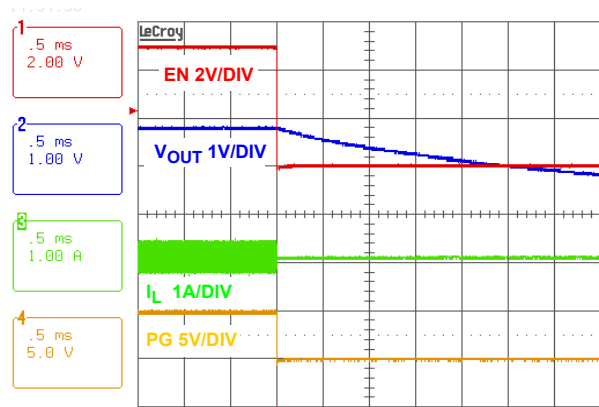
FIGURE 38. SOFT-DISCHARGE SHUTDOWN
