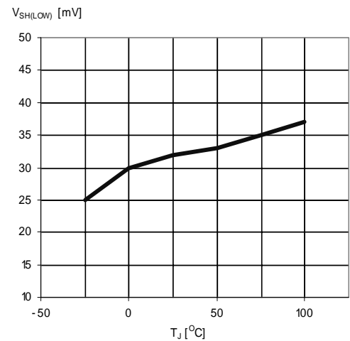
Figure 6. Max. share bus voltage at no load
