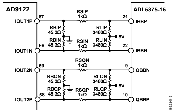
Figure 74. Passive, Level-Shifting Network for Biasing the ADL5375-15
