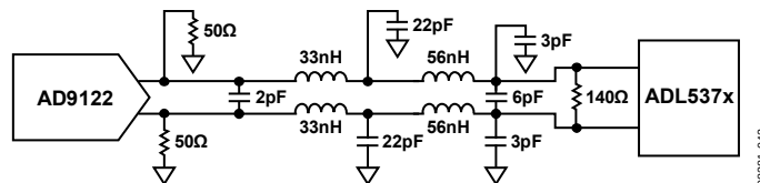
Figure 75. DAC Modulator Interface with Fifth-Order, Low-Pass Filter
