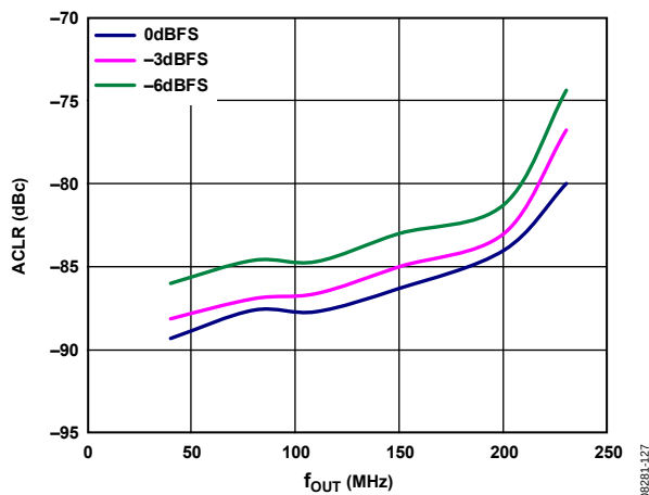
Figure 30. One-Carrier W-CDMA ACLR vs. f_{OUT} over Digital Scale, Second Alternate Channel, PLL Off
