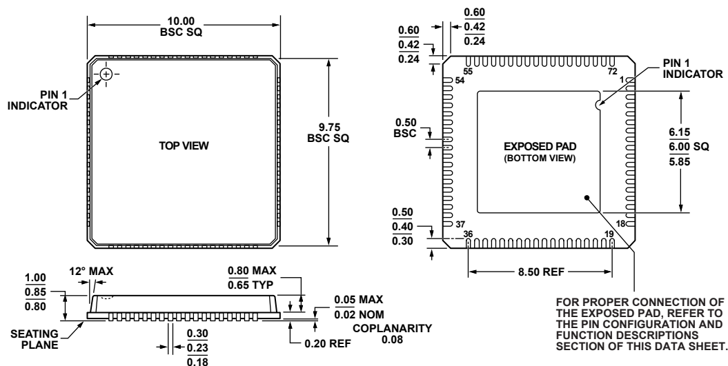
Figure 89. 72-Lead Lead Frame Chip Scale Package [LFCSP_VQ] 10 mm x 10 mm Body, Very Thin Quad (CP-72-7)
