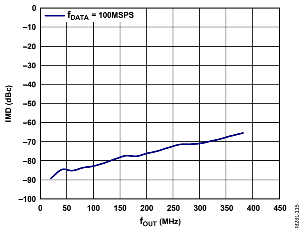
Figure 18. IMD vs. f_{OUT} , 8× Interpolation, f_{DATA} = 100 MSPS, Digital Scale = 0 dBFS, I_{FS} = 20 mA
