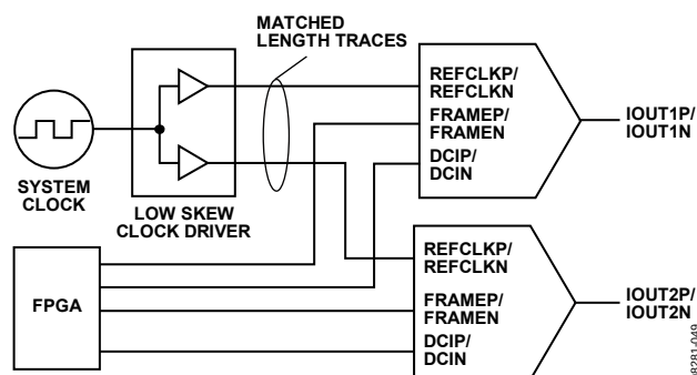
Figure 81. Typical Circuit Diagram for Synchronizing Devices
