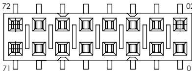
FIGURE 7 POLARIZING POSITIONS
