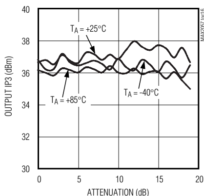
OUTPUT IP3 vs. ATTENUATION
