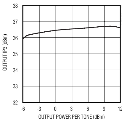
OUTPUT IP3 vs. OUTPUT POWER
