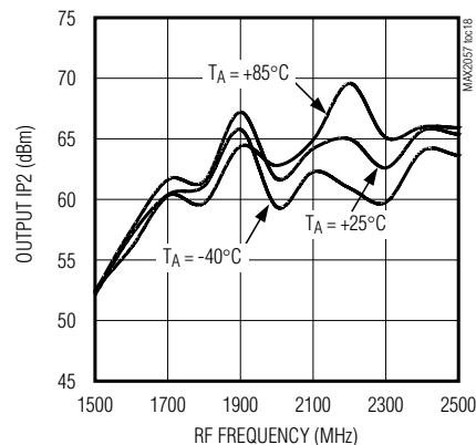
OUTPUT IP2 vs. RF FREQUENCY
