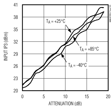
INPUT IP3 vs. ATTENUATION
