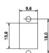
Hole pattern
