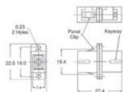
SC duplex coupling
