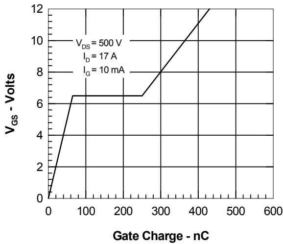
Figure 7. Gate Charge
