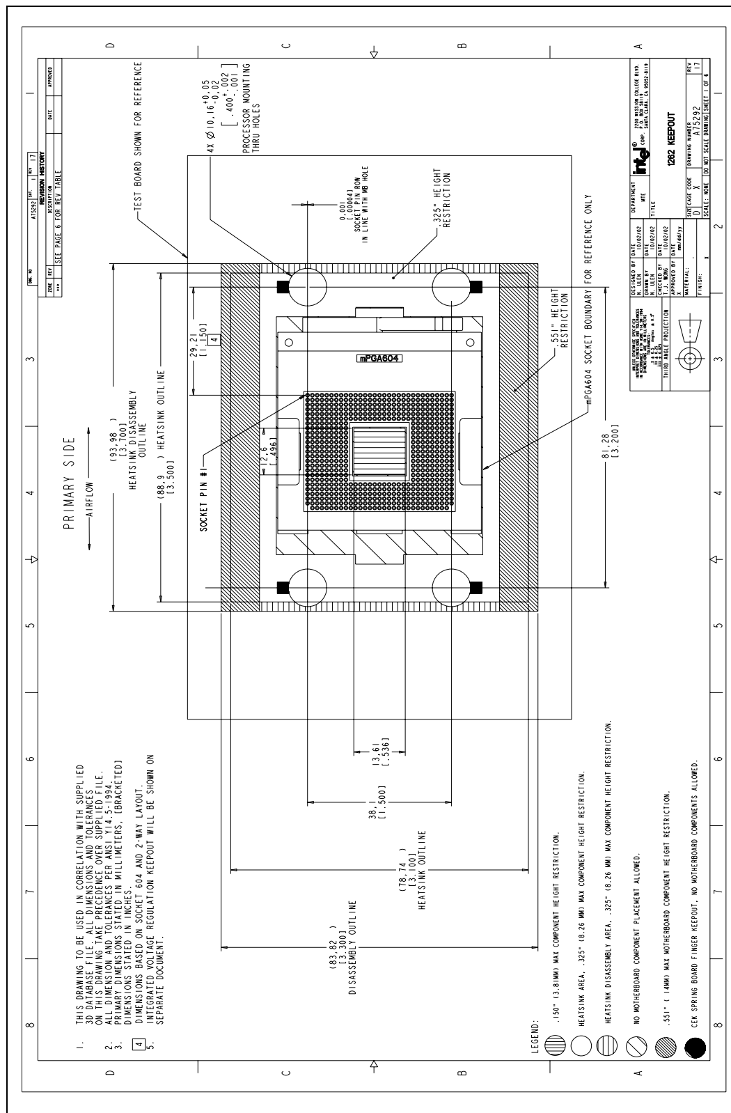
Figure 3-4. Top Side Board Keepout Zones (Part 1)
