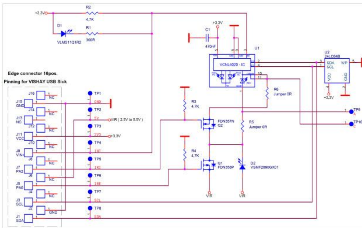
Fig. 8 - Circuit diagramm of VCNL4020 Sensor Board
