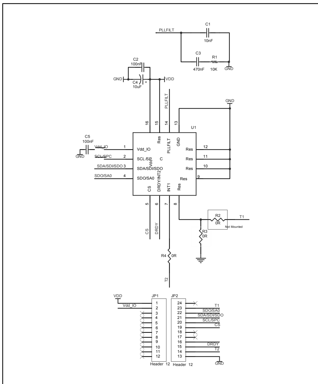
Figure 1: STEVAL-MKI125V1 circuit schematic
