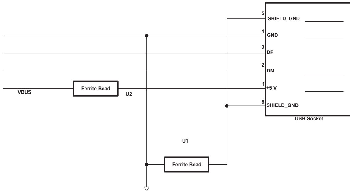
Figure 8-32. USB Connector
