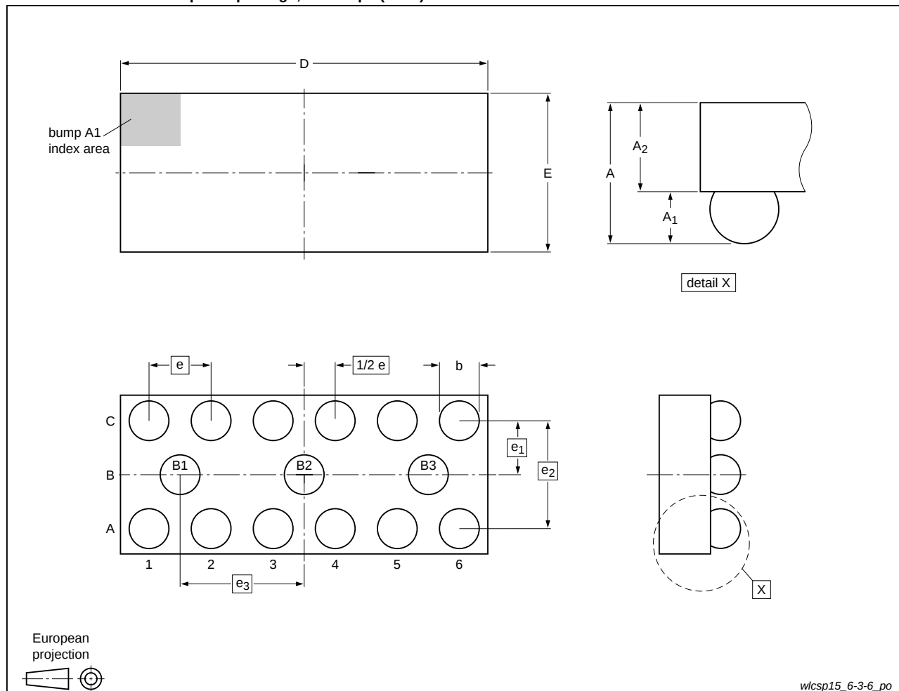
WLCSP15: wafer level chip-size package; 15 bumps (6-3-6)
