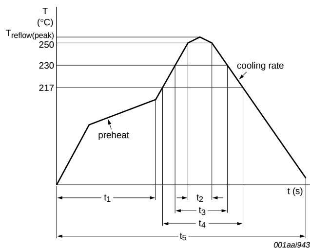
Fig 14. Pb-free solder reflow profile
