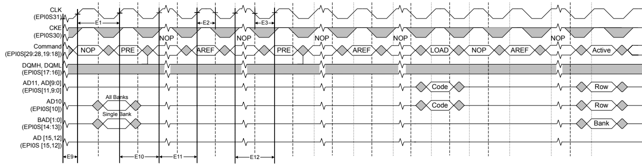
Figure 26-12. SDRAM Initialization and Load Mode Register Timing
