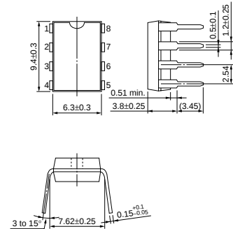
DIP008-P-0300B
