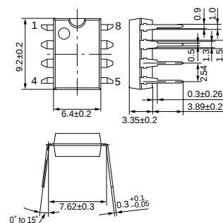
DIP008-P-0300
