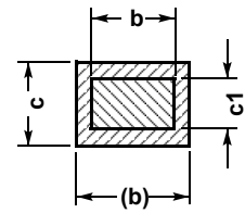
SECTION G-G
