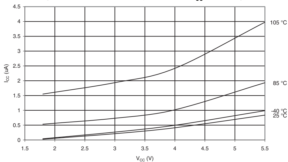
Figure 28-48. ATmega324P: Power-down Supply Current vs. V_{CC} (Watchdog Timer Disabled)
