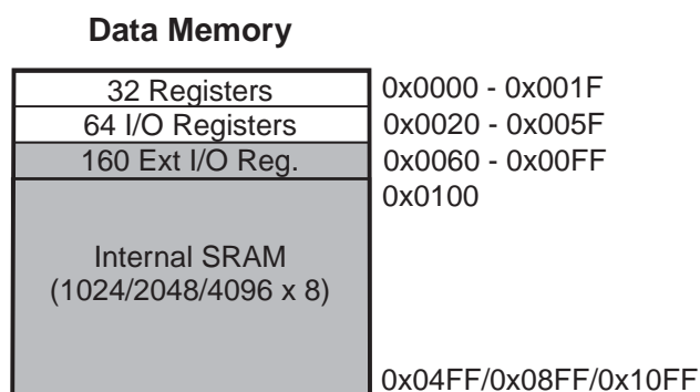
Figure 5-2. Data Memory Map for ATmega164P/324P/644P.
