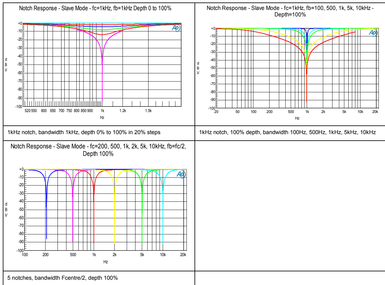
Figure 16 Notch Filter Responses
