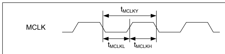
Figure 2 Master Clock Timing
