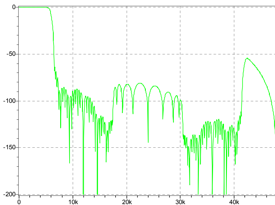
Figure 57 DAC Frequency Response up to 4 \times f_s (Sample rate, f_s = 8\text{ k} to 12\text{ kHz} )
