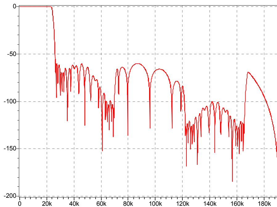
Figure 51 ADC Frequency Response up to 4 \times f_s (Sample rate, f_s = 48\text{kHz} )
