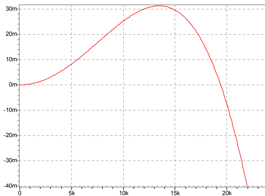
Figure 52 ADC Pass Band Frequency Response up to f_s/2 (Sample rate, f_s = 48\text{kHz} )
