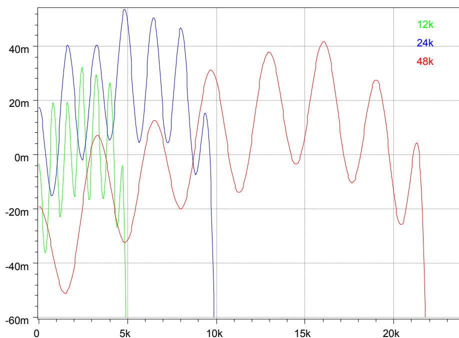
Figure 58 DAC Pass Band Frequency Response up to f_s/2 (Sample rate, f_s = 8\text{ k} to 12\text{ kHz} , 16\text{ k} to 24\text{ kHz} , 32\text{ k} to 48\text{ kHz} )
