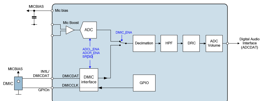
Figure 11 Digital Microphone Interface
