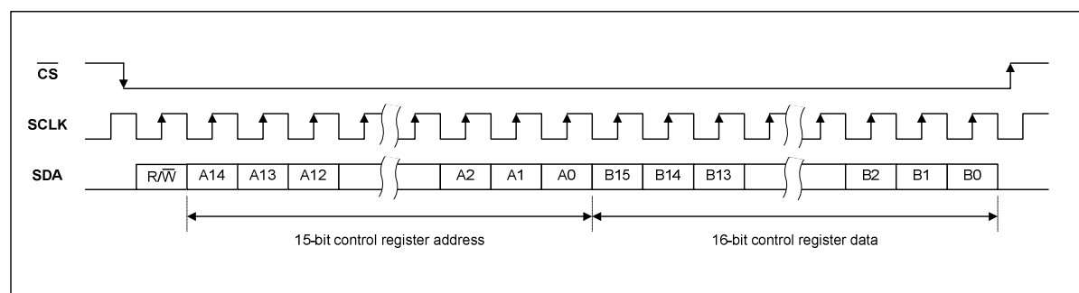
Figure 46 3-Wire Serial Control Interface
