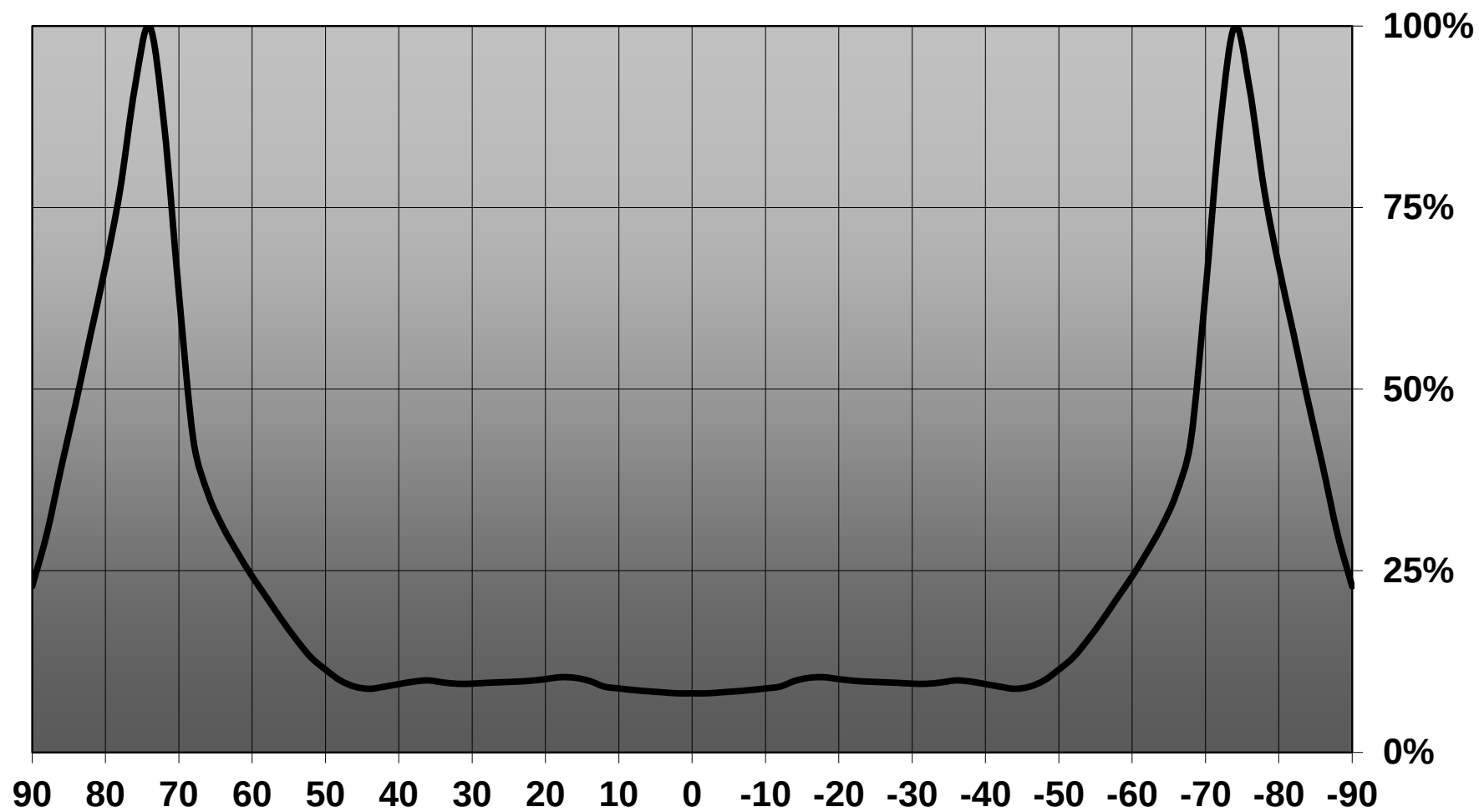
Relative intensity of Strada-S-14_(Oslon_SQ_EC)
