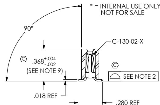
SECTION "A"- "A" STYLE -02
