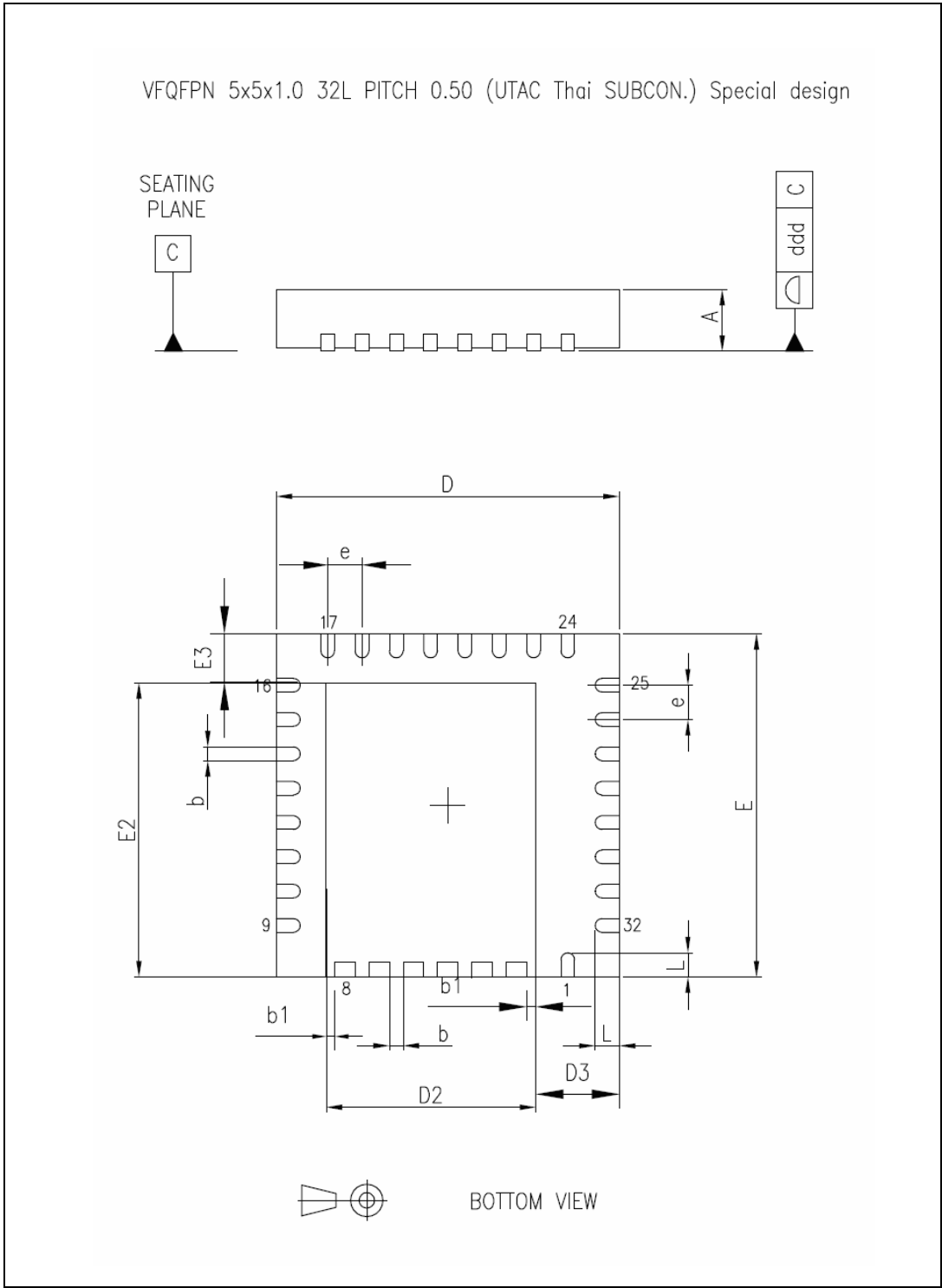
Figure 25. Package dimensions
