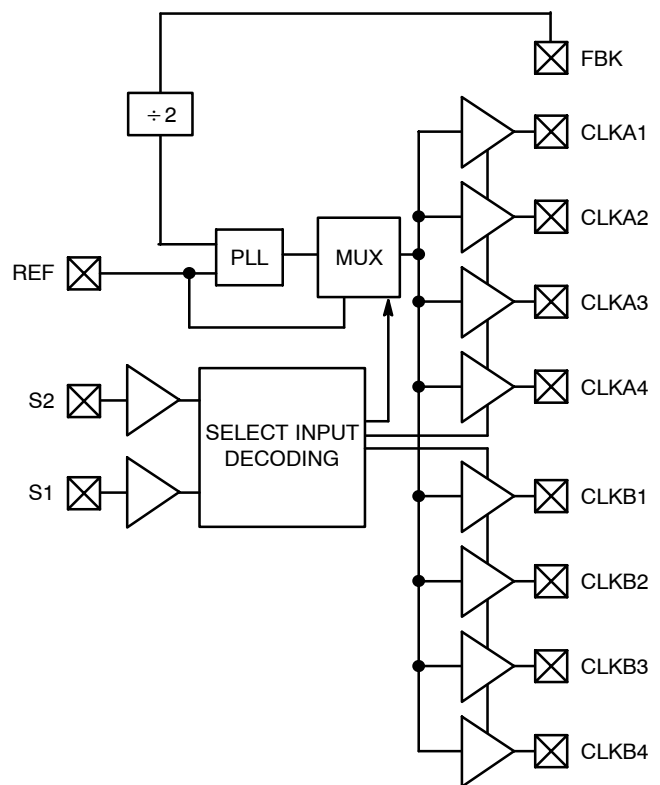
Figure 14. NB2308Ax4
