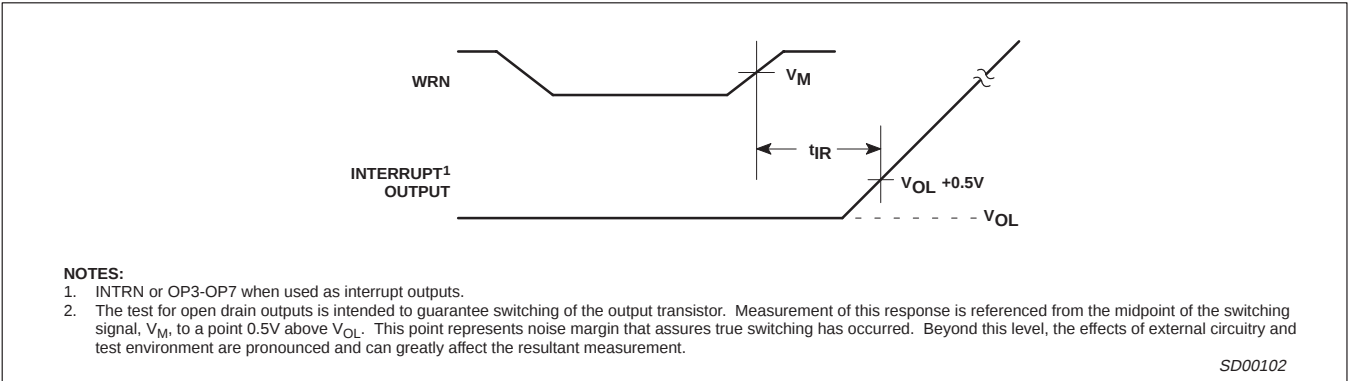
Figure 6. Interrupt Timing
