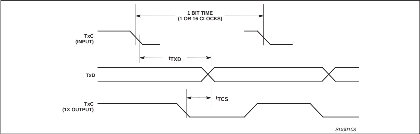
Figure 8. Transmit
