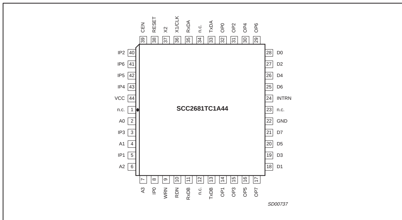
Figure 2. Pin configuration
