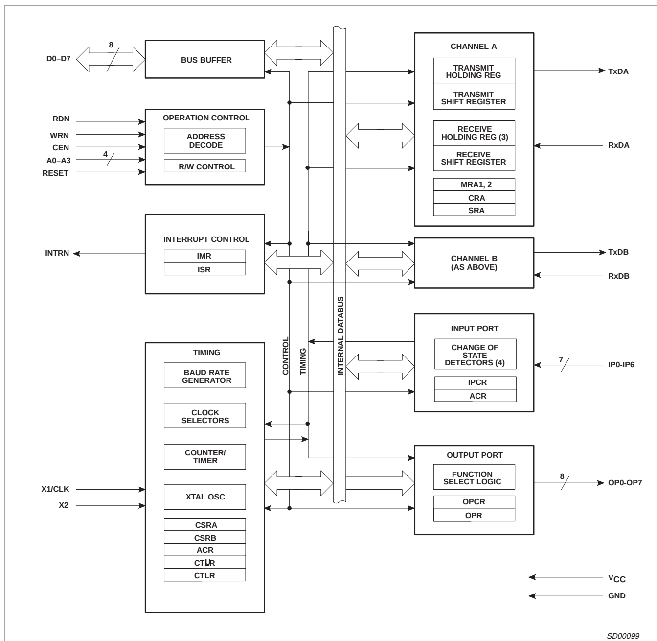
Figure 1. Block Diagram
