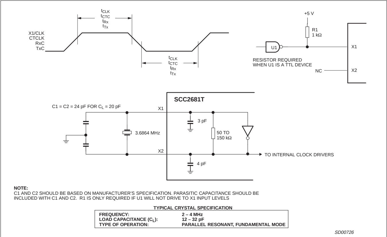
Figure 7. Clock Timing
