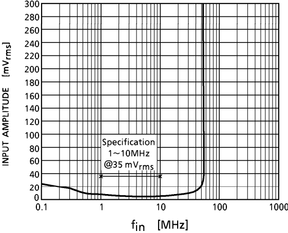
Typical TC9328AF product Input sensitivity LF mode (VDD = 1.5 V, Ta = 25°C)
