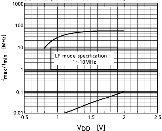
Typical TC9328AF product Input sensitivity LF mode VDD - fmax/fmin (Vin = 35 mVrms, Ta = 25°C)
