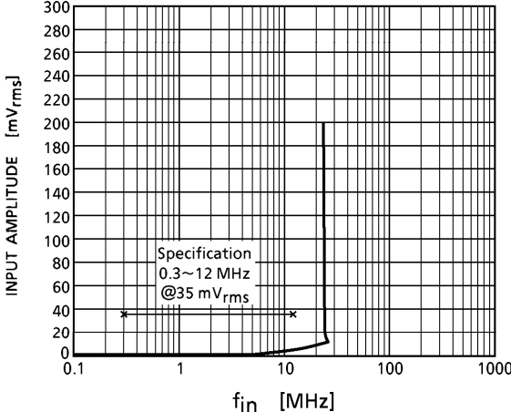
Typical TC9328AF product Input sensitivity IFin mode (VDD = 1.5 V, Ta = 25°C)
