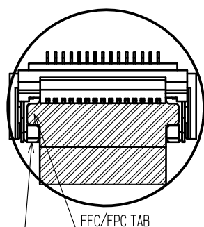
Guide for positioning FFC/FPC
