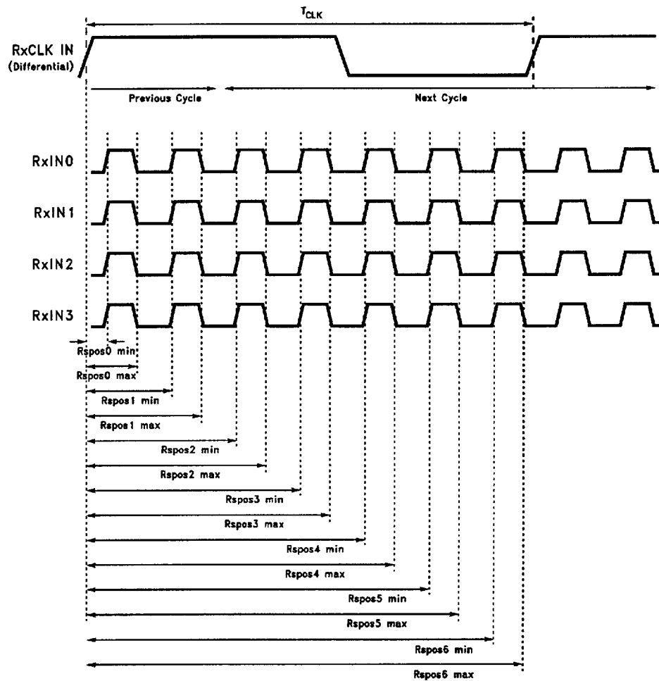
FIGURE 17. Receiver LVDS Input Strobe Position
