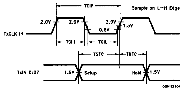
FIGURE 6. DS90CR285 (Transmitter) Setup/Hold and High/Low Times
