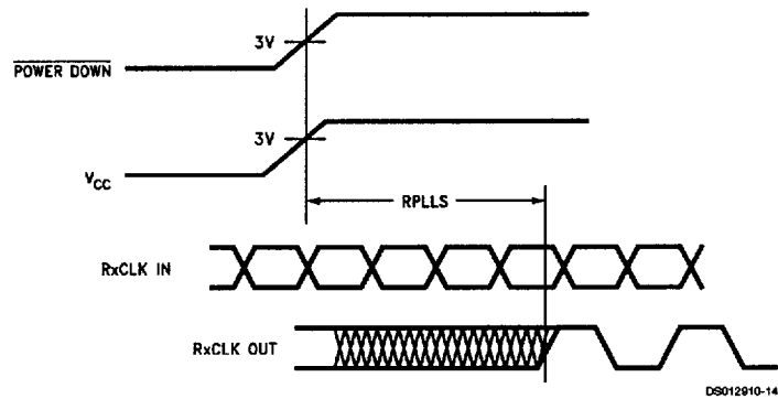
FIGURE 11. DS90CR286 (Receiver) Phase Lock Loop Set Time
