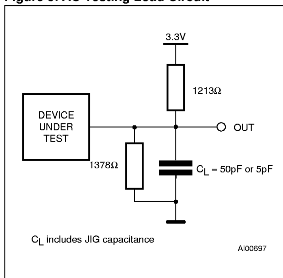
Figure 3. AC Testing Load Circuit
