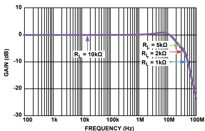
FIGURE 40. FREQUENCY RESPONSE vs LOAD RESISTANCE
