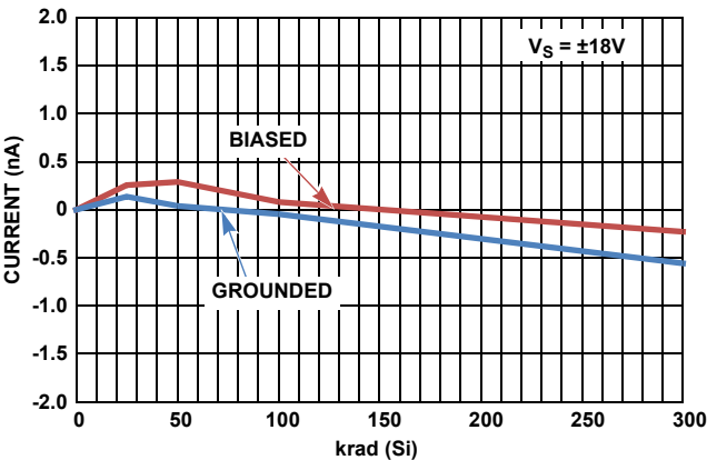
FIGURE 56. I_{OS} SHIFT vs HIGH DOSE RATE RADIATION
