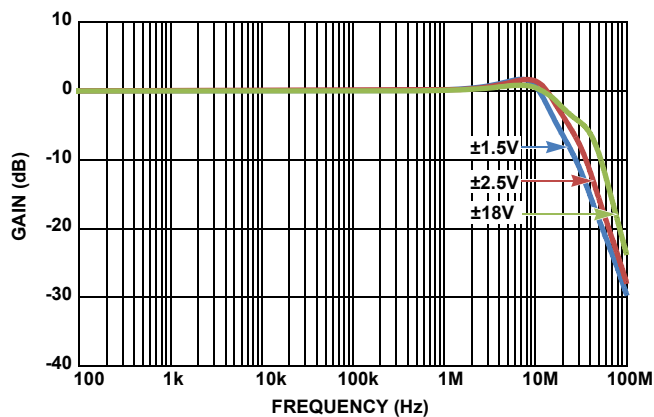
FIGURE 42. FREQUENCY RESPONSE vs SUPPLY VOLTAGE
