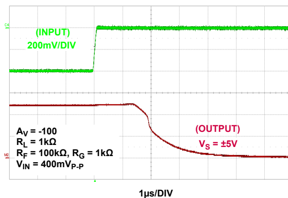
FIGURE 48. SATURATION RECOVERY ( V_S = \pm 5V )
