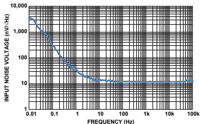
FIGURE 27. INPUT NOISE VOLTAGE SPECTRAL DENSITY ( V_S = \pm 18V )
