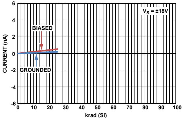
FIGURE 59. I_{OS} SHIFT vs LOW DOSE RATE RADIATION
