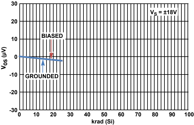
FIGURE 57. V_{OS} SHIFT vs LOW DOSE RATE RADIATION
