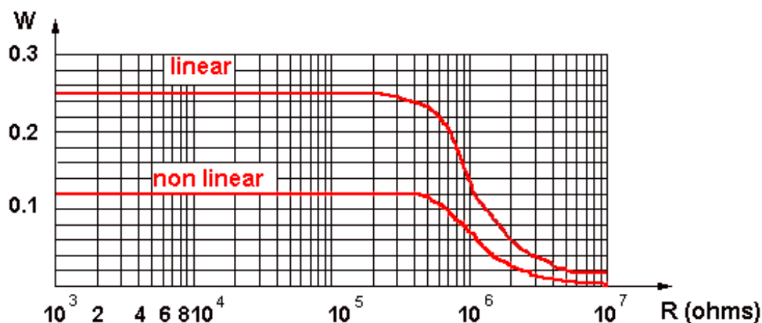
MAXIMUM WORKING VOLTAGE CURVE:
