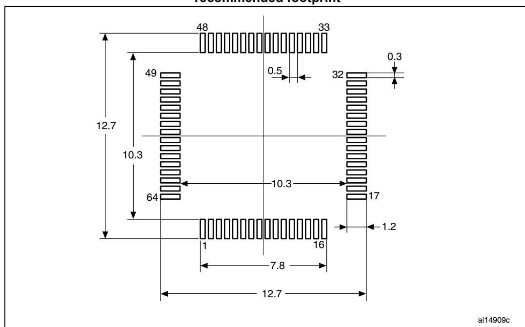
Figure 37. LQFP64, 10 x 10 mm, 64-pin low-profile quad flat package recommended footprint
