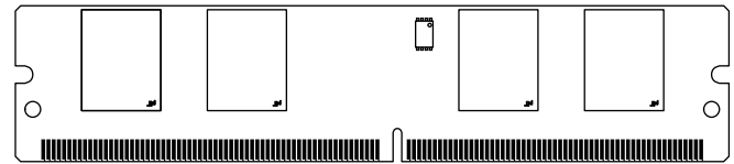
Figure 1: 244-Pin ULP Mini-UDIMM
