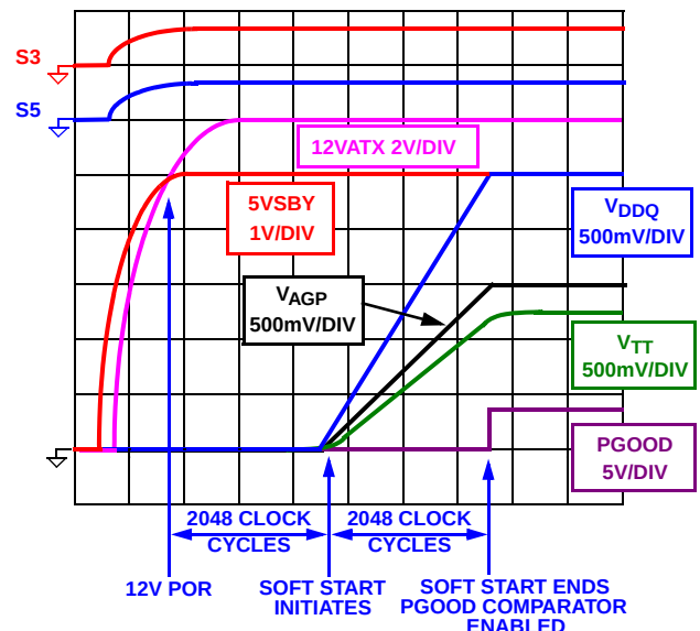
FIGURE 1. TYPICAL COLD START
