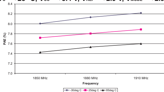
Figure 6: PAE vs. Frequency
