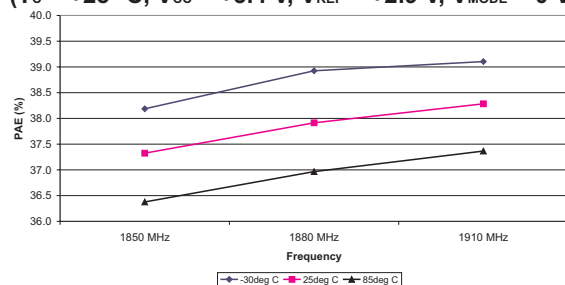
Figure 3: PAE vs. Frequency
