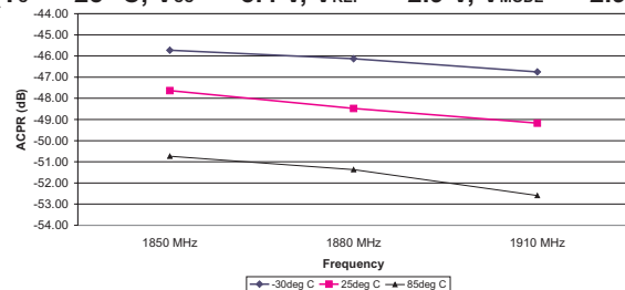
Figure 7: ACP1 vs. Frequency
