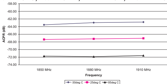
Figure 8: ACP2 vs. Frequency
