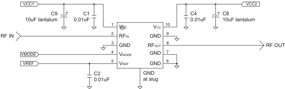
Figure 12: Application Circuit Schematic
