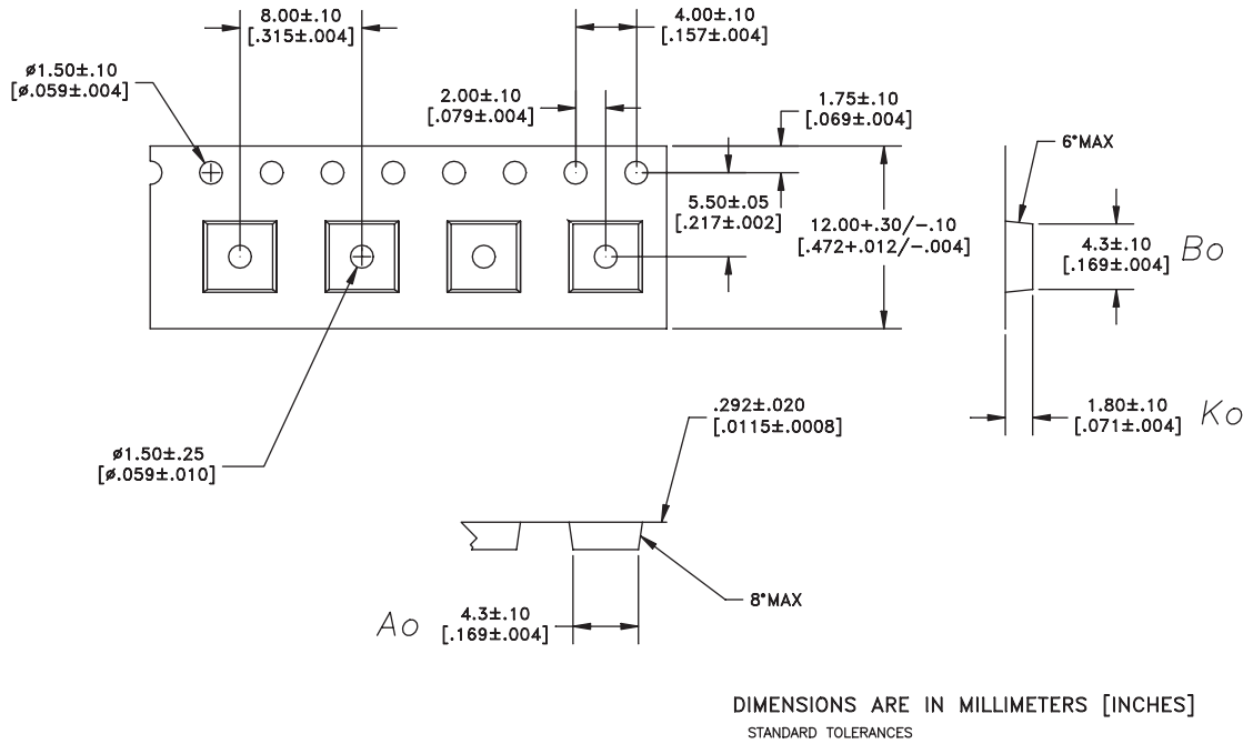
Figure 15: Tape & Reel Packaging
