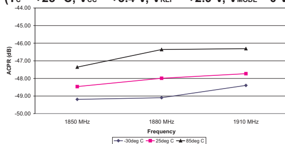
Figure 4: ACP1 vs. Frequency
