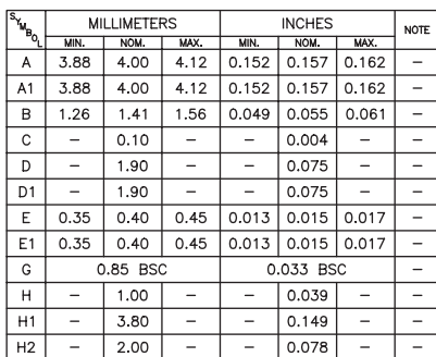
Figure 13: M7 Package Outline - 10 Pin 4mm x 4mm Surface Mount Module
