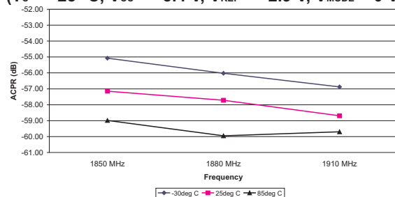
Figure 5: ACP2 vs. Frequency
