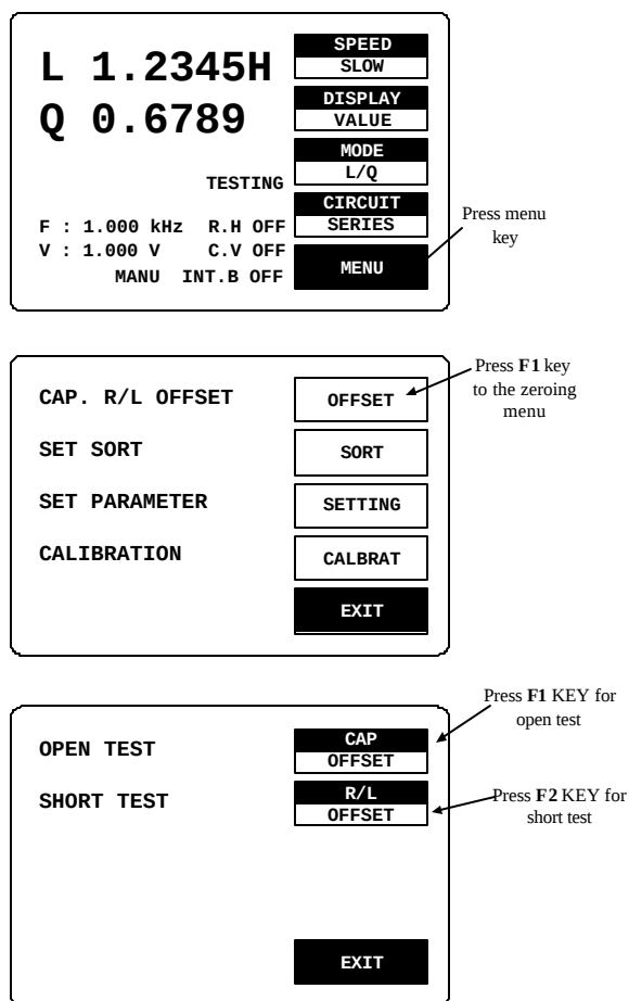
Figure 4-1: Summary of zeroing menu
