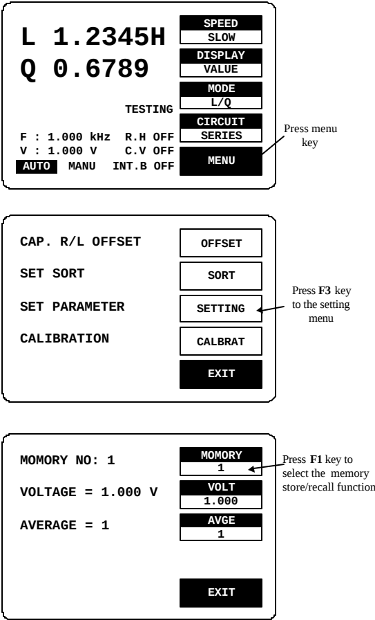
Figure 4-12. Programming of memory store/recall.
