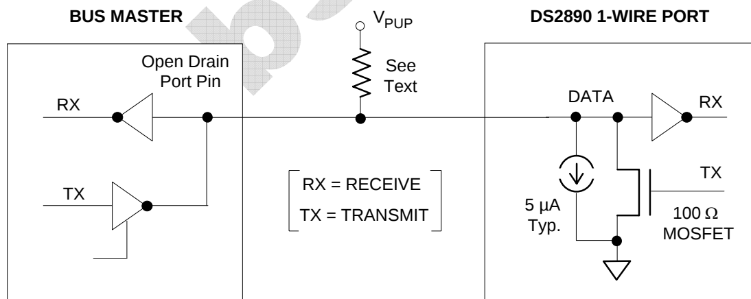
FIGURE 14. HARDWARE CONFIGURATION
