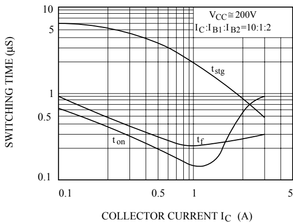
SWITCHING CHARACTERISTICS
