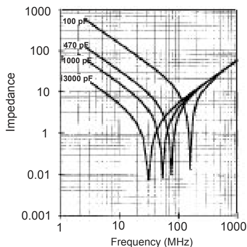
CDV16 Impedance vs. Frequency
