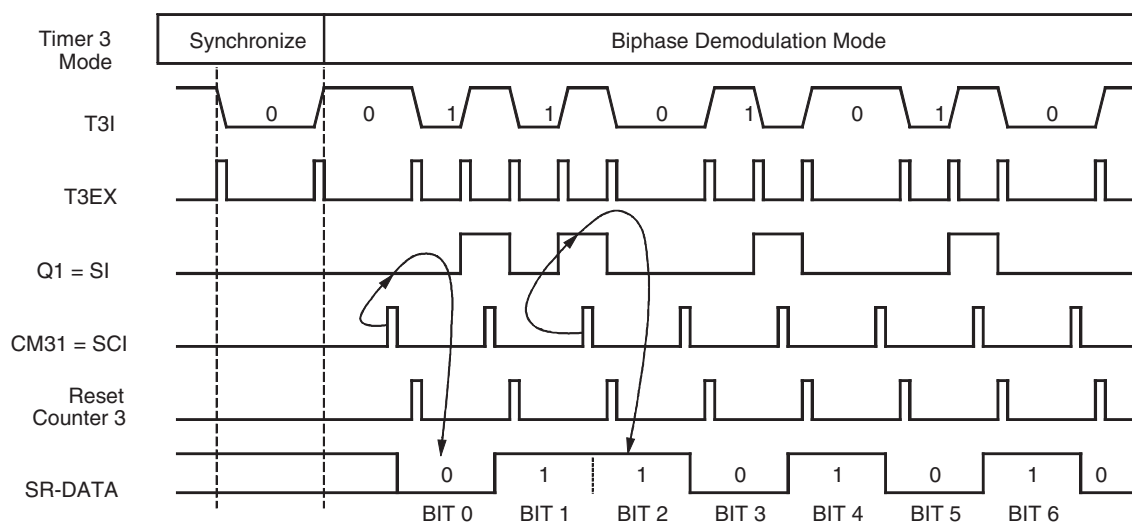
Figure 5-57. Bi-phase Demodulation
