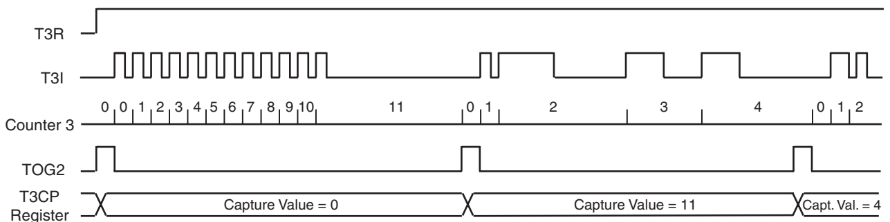
Figure 5-29. Event Counter with Time Gate
