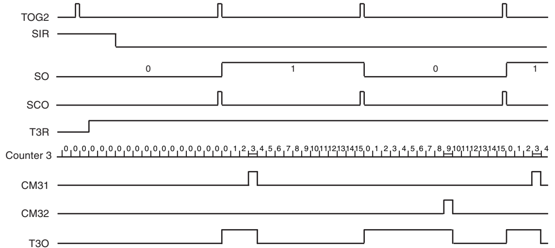
Figure 5-31. Pulse-width Modulation
