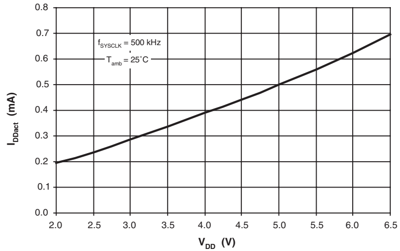
Figure 13-3. Active Supply Current versus V_{DD}
