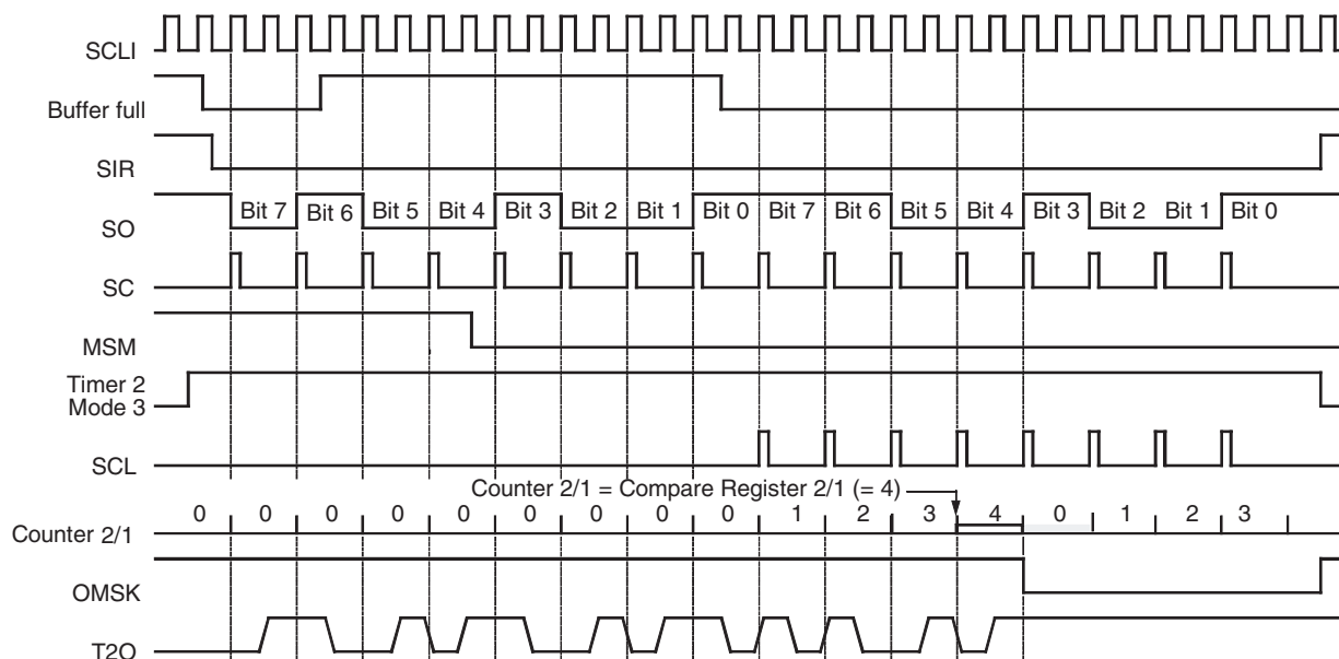
Figure 5-51. Manchester Modulation 2
