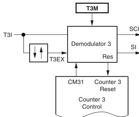
Figure 5-36. Timer 3 – Demodulator 3
