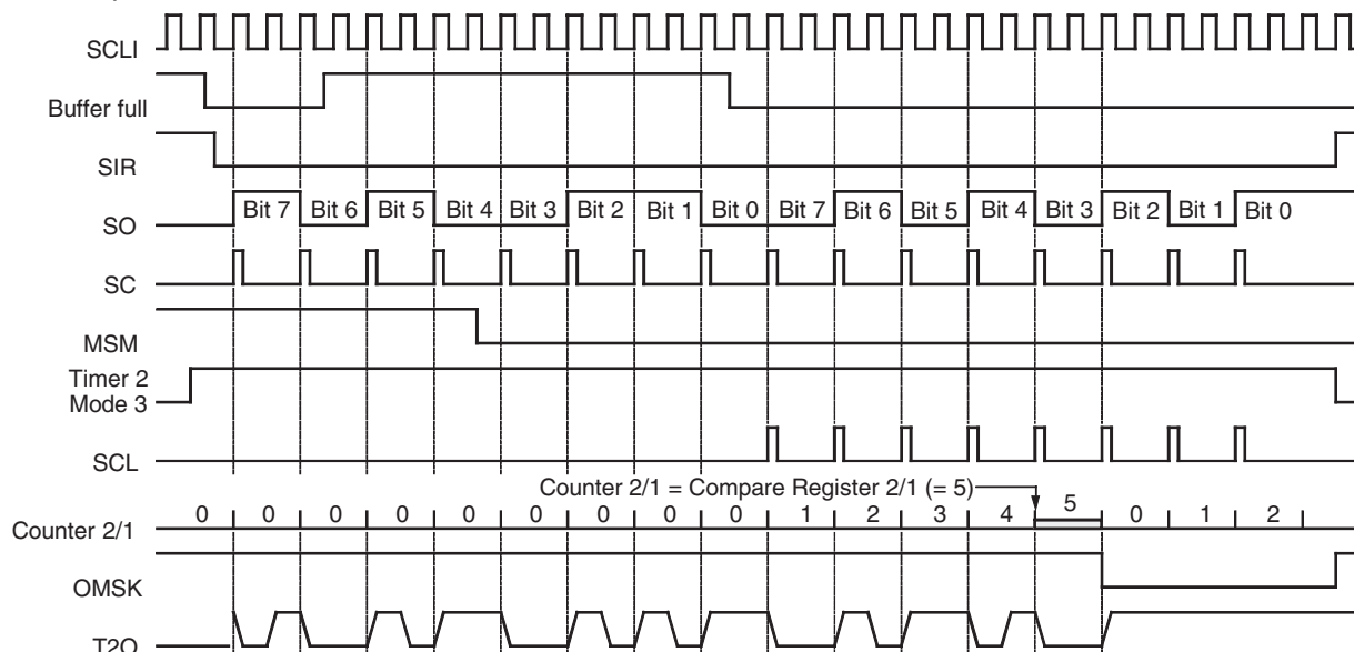
Figure 5-52. Bi-phase Modulation 2
