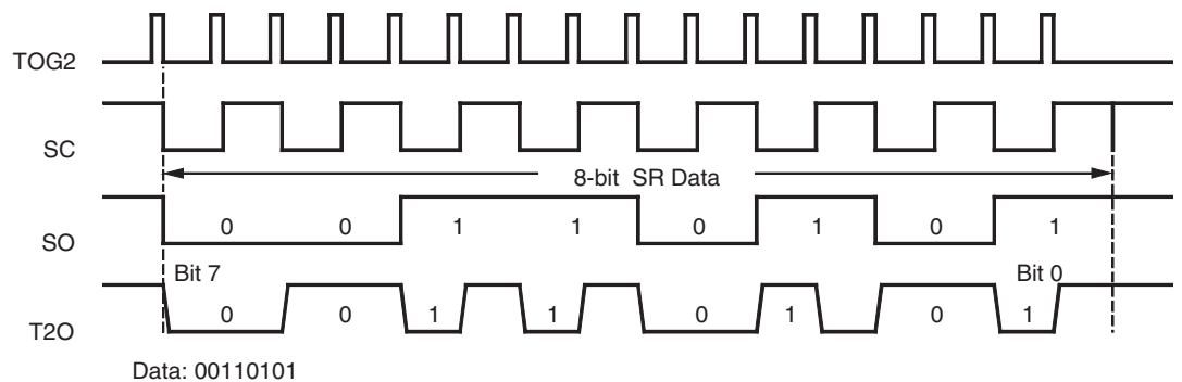
Figure 5-49. Bi-phase Modulation 1
