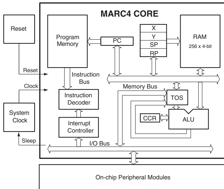
Figure 4-1. MARC4 Core
