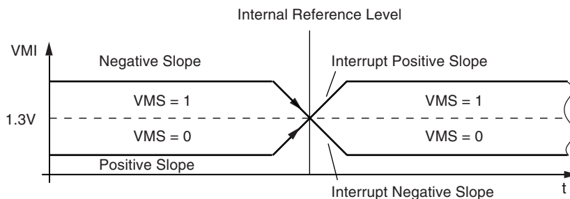
Figure 4-11. External Input Voltage Supervisor
