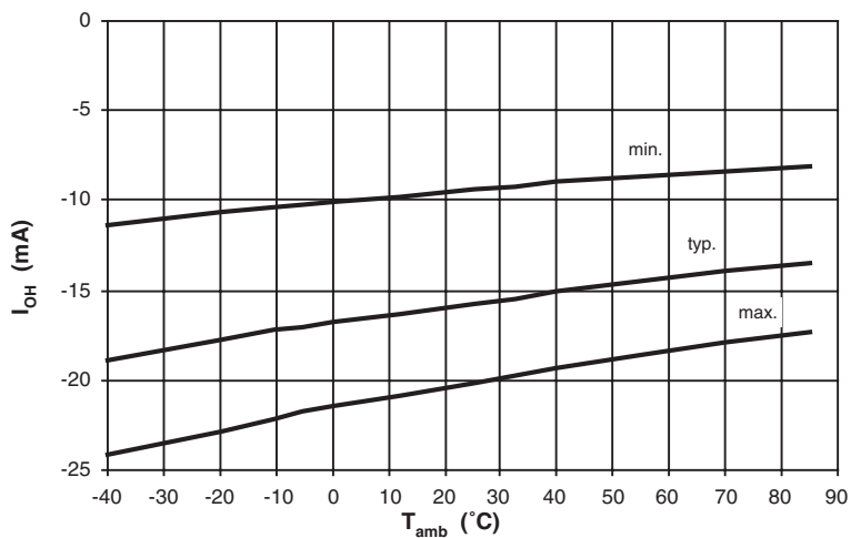
Figure 13-20. Output High Current versus T_{amb} , V_{DD} = 6.5 V , V_{OH} = 0.8 \times V_{DD}
