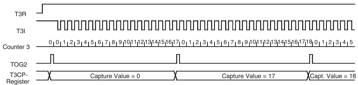
Figure 5-59. Frequency Measurement
