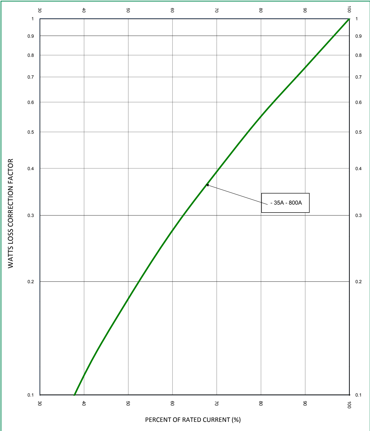
Watts Loss Correction Factor Curve L70QS Series
