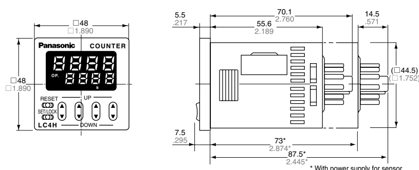
Pin type (Flush mount/Surface mount)
