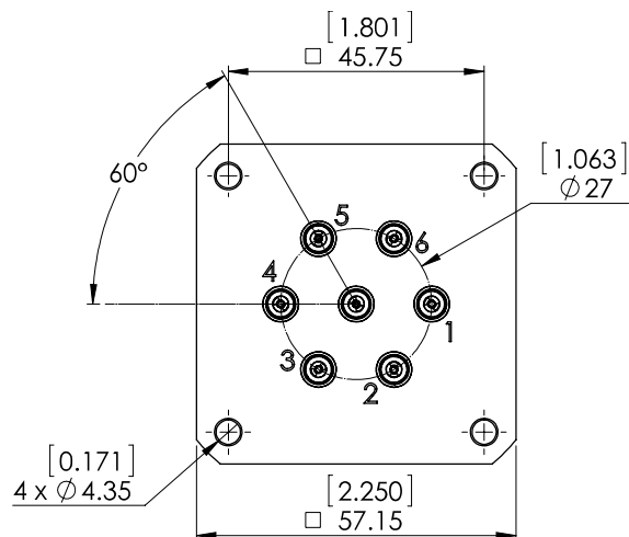
SMA 2.9 Connectors
