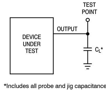
Figure 2. Test Circuit
