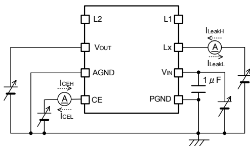
< Circuit No.⑦ >
