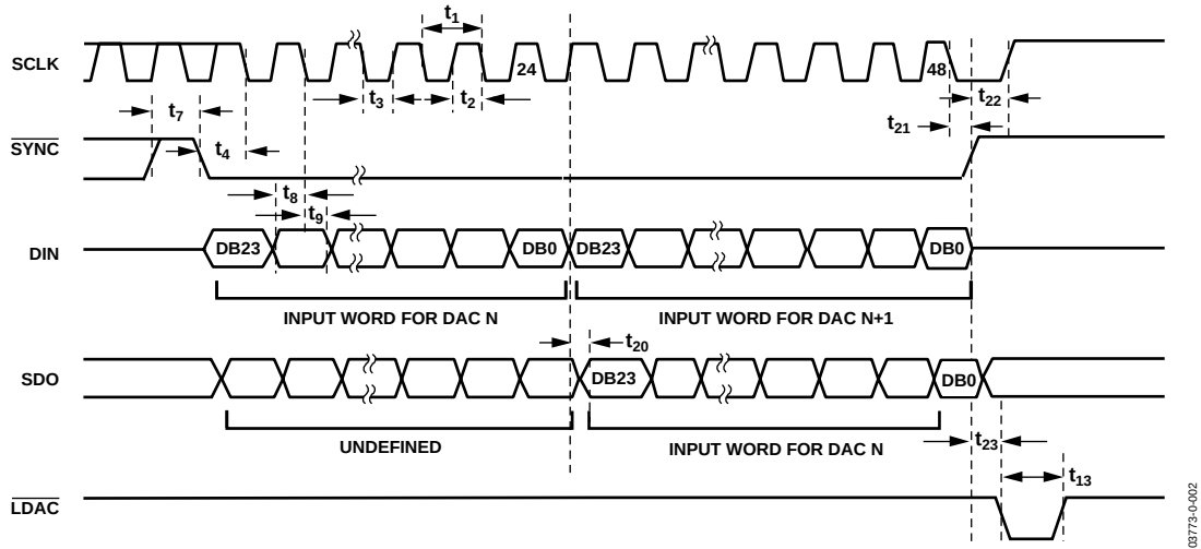
Figure 2. Serial Interface Timing Diagram (Daisy-Chain Mode)
