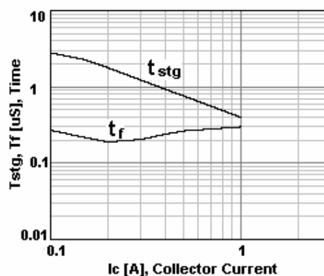
Figure 4. Switching Time
