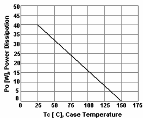
Figure 6. Power Derating
