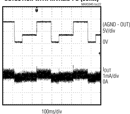
DETECTION WITH INVALID PD ( 33k\Omega )
