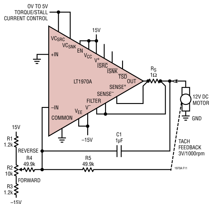
Figure 11. Simple Bidirectional DC Motor Speed Controller
